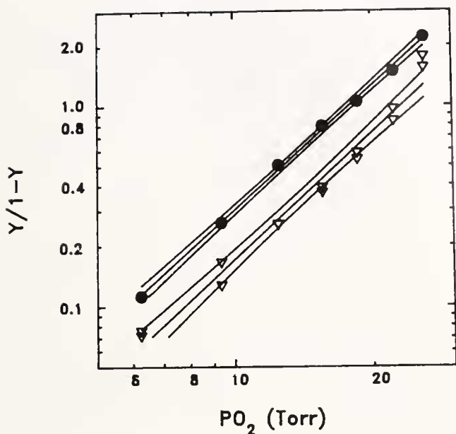
Figure 2. Hill plots of O_2 binding properties of isolated hexamers and dodecamers. 25^\circ C , 0.05 \text{ mol l}^{-1} Tris buffered saline containing 10 \text{ mmol l}^{-1} CaCl_2 , 25 \text{ mmol l}^{-1} MgCl_2 , and 300 \text{ mmol l}^{-1} NaCl . Tonometric data for one aliquot of hexamers (circles, pH 7.49) and two of dodecamers (triangles, pH 7.52). Lines are regression lines and their 95% confidence intervals.
